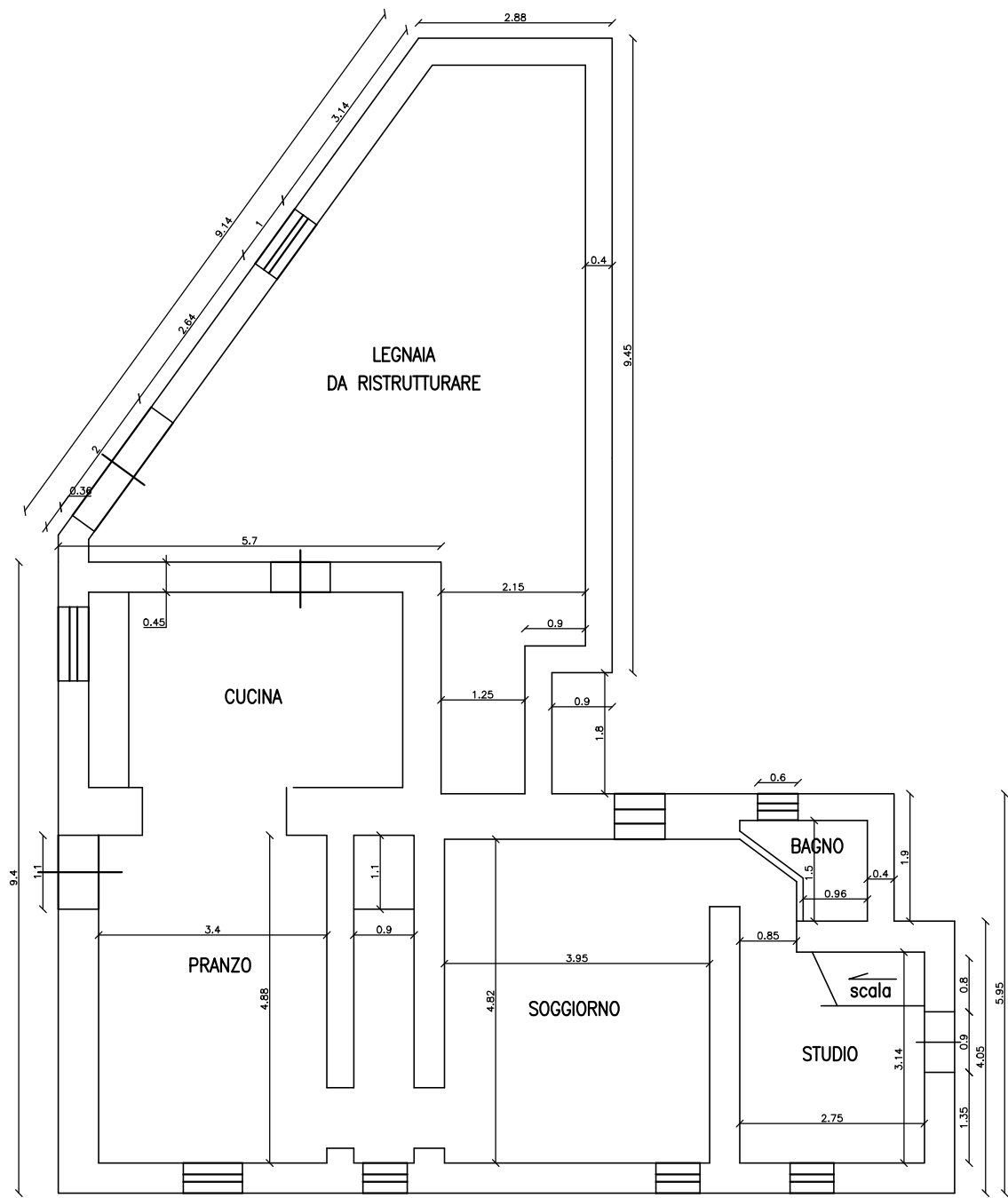
PIANO TERRA
