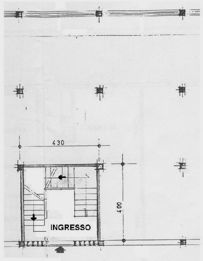
PIANO TERRA
